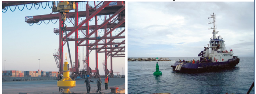
Sealite Poseidon Buoy installation, fitted up with an SLC310 light-head, Sint Maarten
